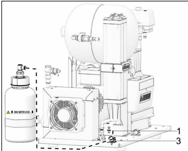
Fig. 7: Condensate drain
