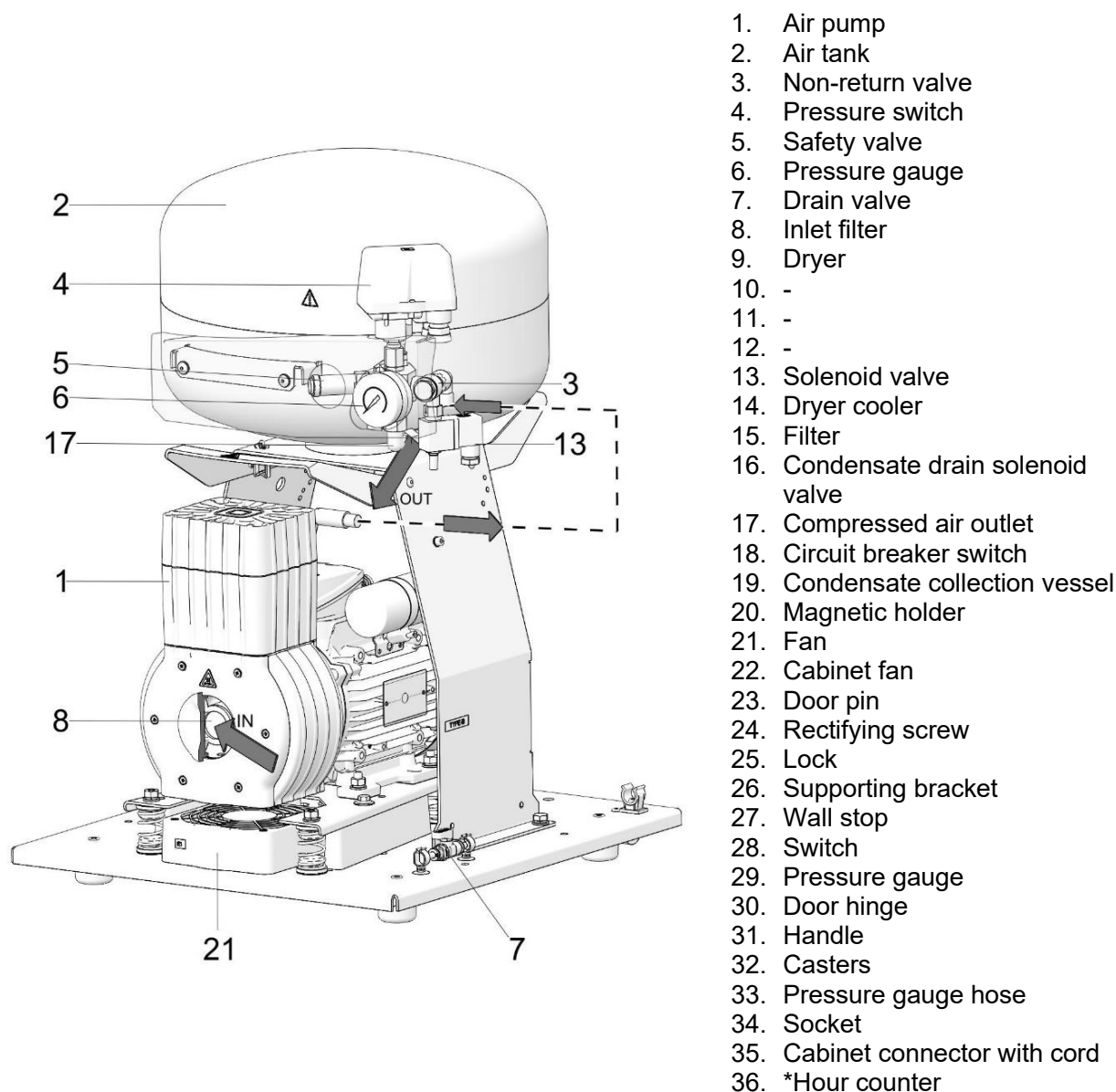
Fig. 1 - DK50 PLUS - Compressor
