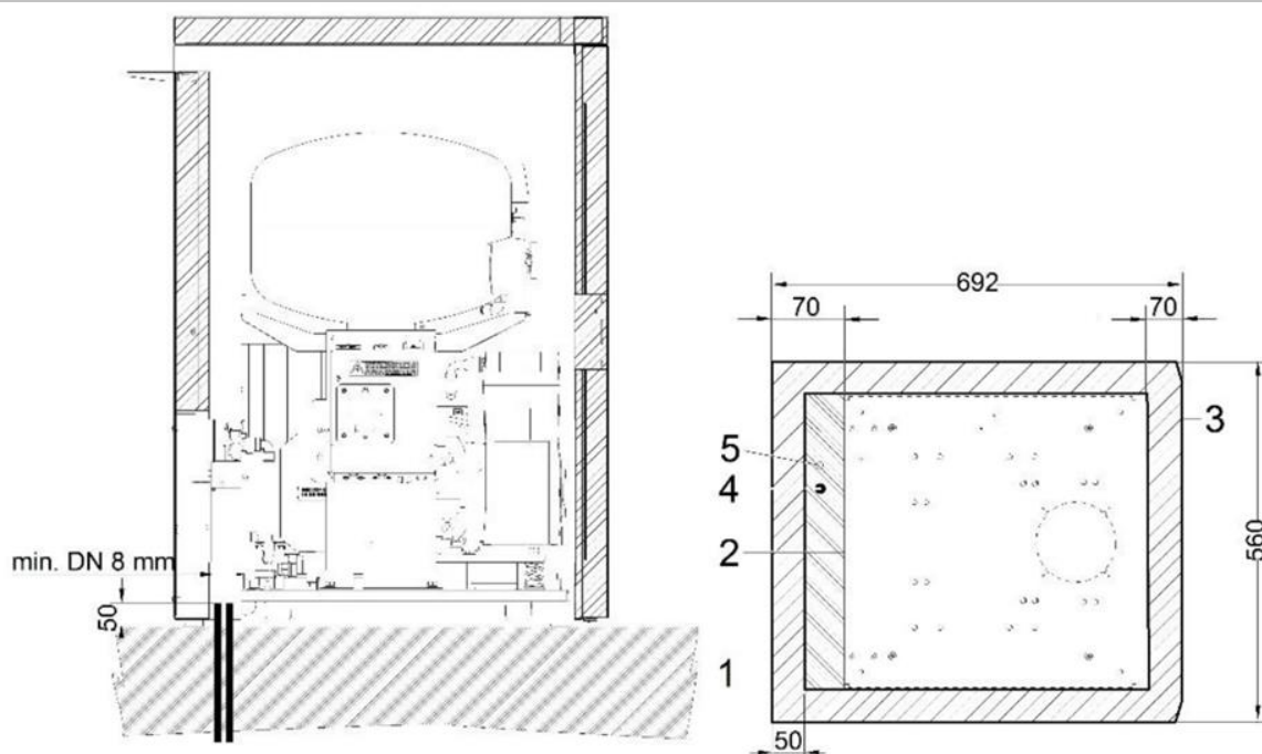
Fig. 9: Floor installation
