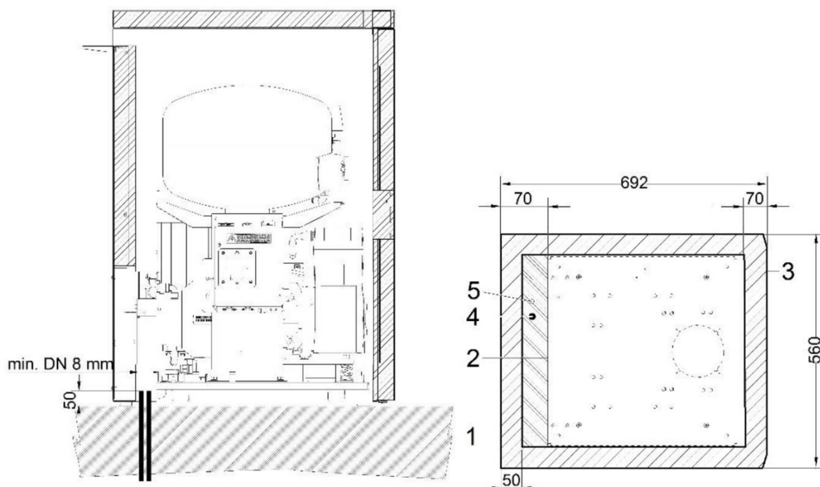
Abb. 9: Bodeninstallation
