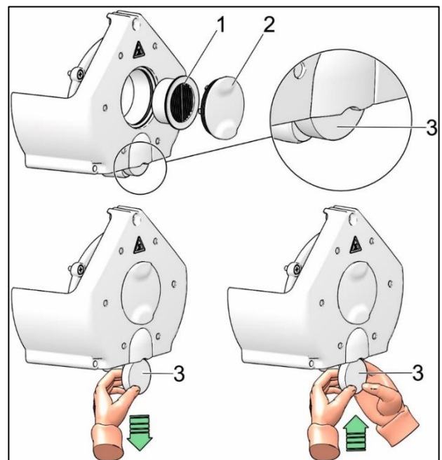
Fig. 21: Inlet filter and pre-filter replacement
