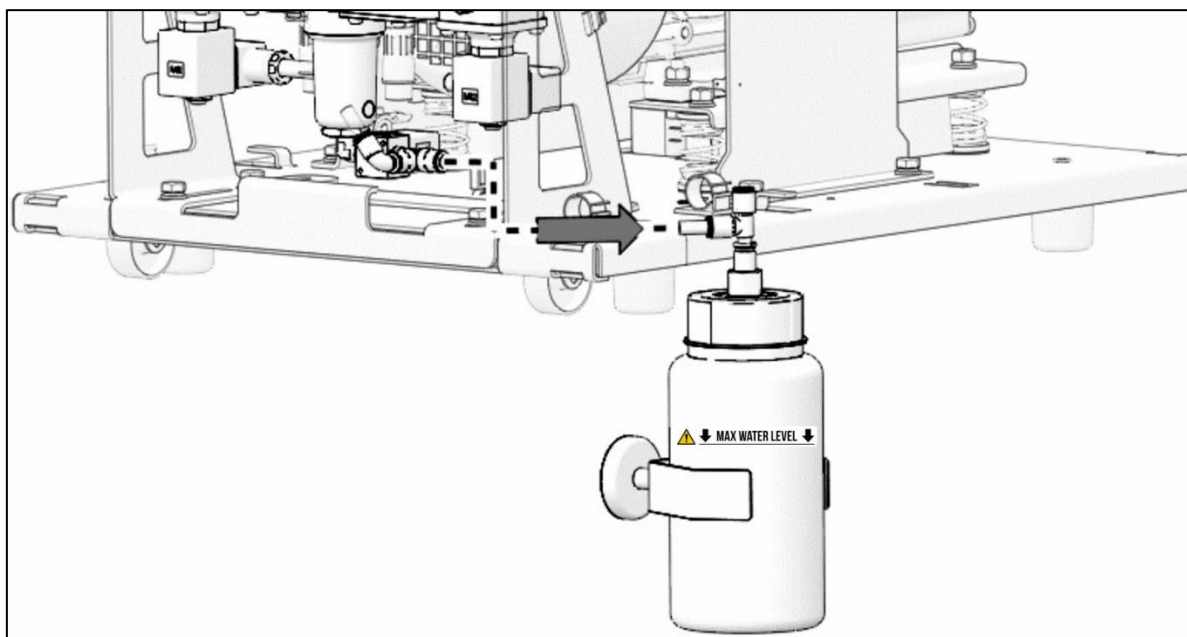
Fig. 8: Connection of condensate collection vessel
